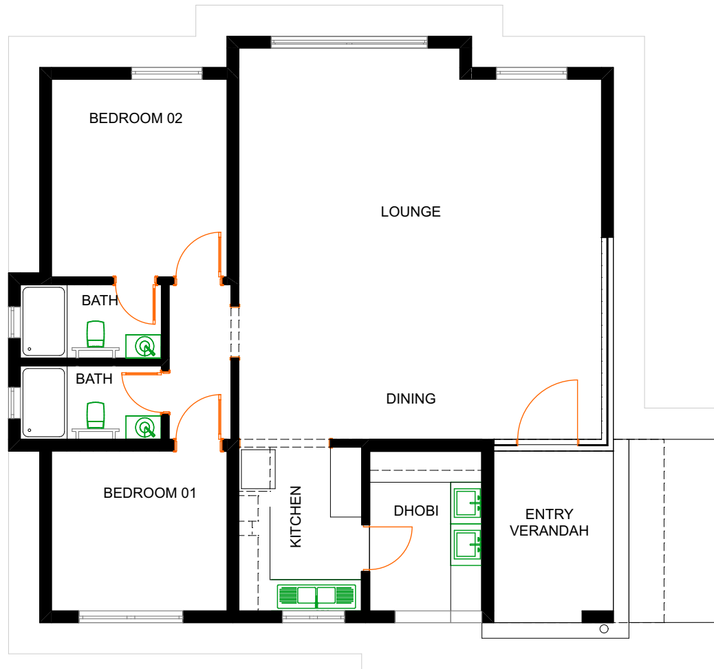
FLOOR PLAN - 2 BEDROOM
